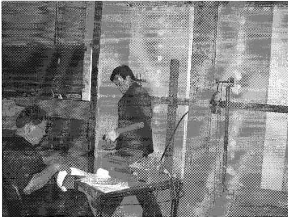
Figure 5 Testing of resistance to crowd pressure.
