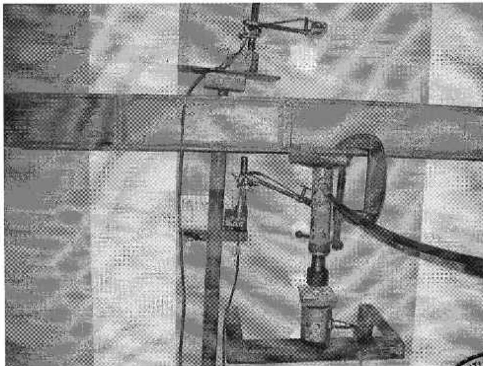
Figure 8 Testing of heavyweight anchorage by eccentric downward loading (wash basin).
