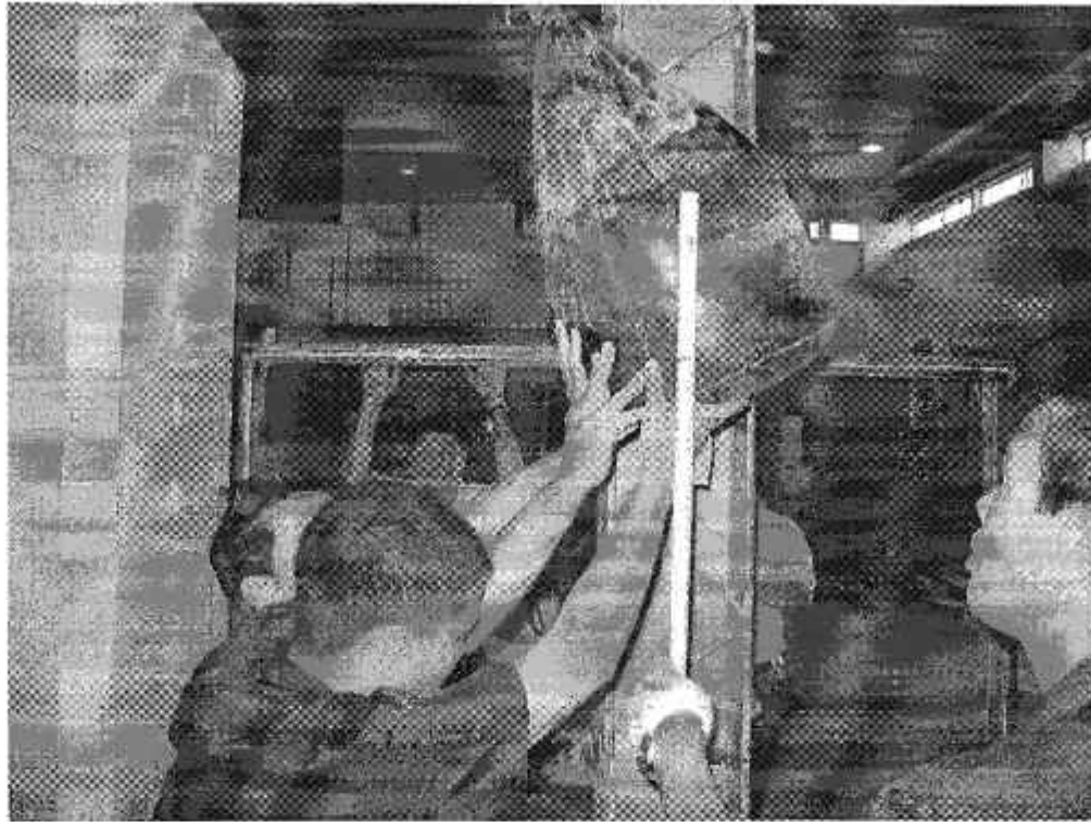
Figure 3 Testing of large soft body impact.
